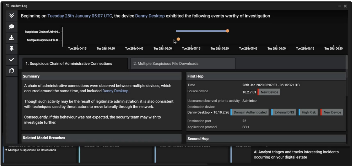
Figure 9: Sample UI image shows Cyber AI Analyst identified unusual administrative activity and file downloads.
